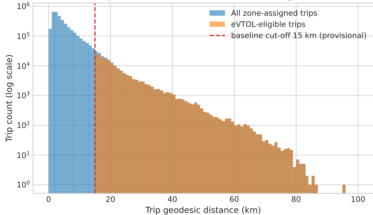
Trip distance distribution: all vs eVTOL-eligible
