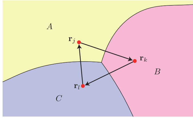
Figure 4.1: Diagram showing the partition of the plane into three regions labelled with A , B and C . An example of h_{jkl} is depicted with red dots, where arrows indicate the positive direction.
