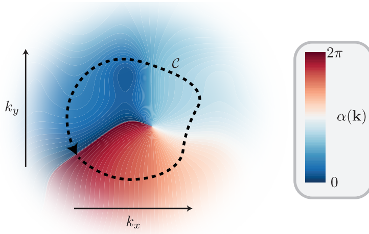
Figure 2.1: An example of a non-smooth gauge transformation designed to change the value of the Berry phase around the path \mathcal{C} – marked with a dashed line – by an addition of 2\pi . Only a small region of \mathbf{k} -space is shown, with the local phase applied shown by the colormap.
