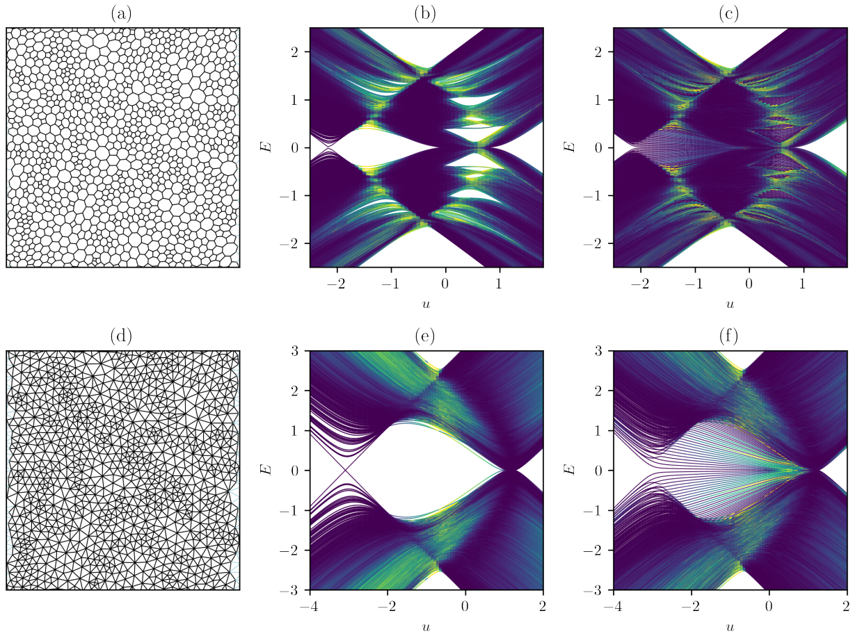
Figure 2.6: Plots showing the spectra of the amorphous QWZ model for two different example lattices. States are coloured according to their inverse participation ratio. (a) A trivalent lattice generated from a Voronoi decomposition of a set of random points, followed by five iterations of Lloyd's algorithm.
