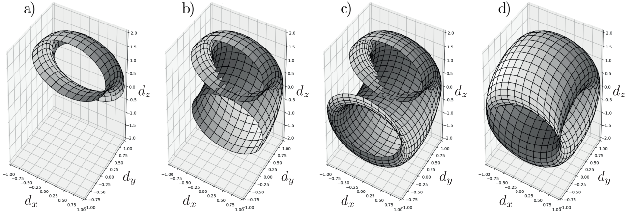
Figure 2.2: The embedding of the Brillouin zone in \mathbf{d} -space for the QWZ model. This is shown in four progressive cutaways to ensure the internal structure can be seen. In all four images k_x spans the interval [0, 2\pi) , however in (a) k_y spans [0, \frac{\pi}{2}) , in (b) k_y spans [0, \pi) , in (c) k_y spans [0, \frac{3\pi}{2}) , and in (d) k_y spans [0, 2\pi) .
