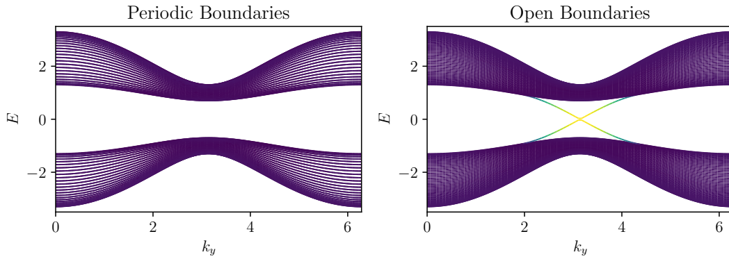
Figure 2.4: An example band structure for a QWZ model with u = 1.3 and L_x = 30 . States are coloured according to their inverse participation ratio, indicating their relative degree of localisation. (Left) The example for periodic boundary conditions, showing two well-separated bands. (Right) The case for open boundary conditions. Two edge states are shown leaving the bulk and crossing the gap, with the descending state being a left edge state, and the ascending state being a right edge state.
