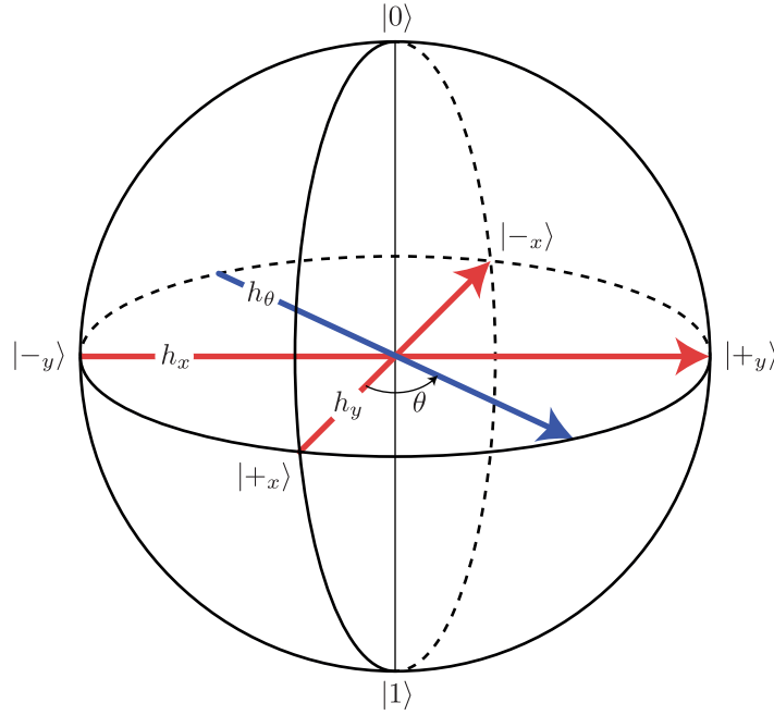
Figure 2.5: The Bloch sphere, showing the positions of the eigenstates of the three Pauli matrices. The action of the hopping matrices is shown in red, where the h_x and h_y operators act as creation operators on the y and x bases respectively. The action of our arbitrary angle hopping operator is shown in blue, acting as a creation operator between a pair of orthogonal states that lie on the x - y plane.
