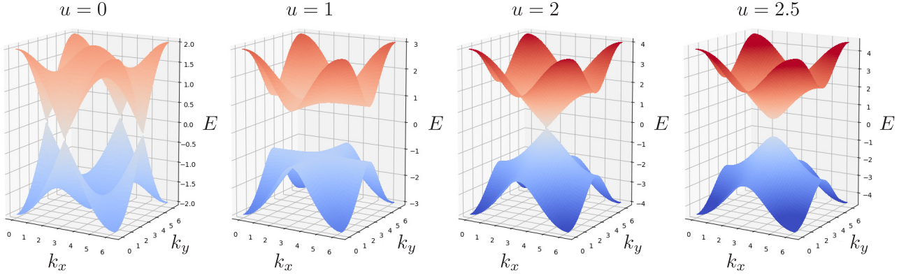
Figure 2.3: Four examples of the band structure of the QWZ model are shown, for varying u values between 0 and 2.5. At u = 0 and 2, the bands touch and Chern number is undefined. At u = 1 , \mathcal{C} = +1 , and at u = 2.5 , \mathcal{C} = 0 .
