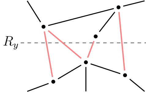
Figure 5.6: A section of amorphous lattice is shown. All hopping terms in the Hamiltonian that cross the line y = R_y acquire a phase given by eqn. 5.41, these are depicted in red. Unaffected hopping terms are shown in black. Note that the phase is ill-defined when a site \mathbf{r}_i lies on the line, however this can be remedied by infinitesimally shifting R_y .
