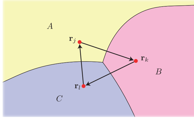
Figure 5.1: Diagram showing the partition of the plane into three regions labelled with A , B and C . An example of h_{jkl} is depicted with red dots, where arrows indicate the positive direction.
