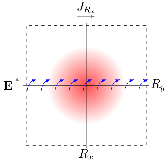
Figure 5.7: A schematic for local Hall measurement. The bottom half of the system has its potential raised with respect to the top half, generating an electric field acting over the horizontal line. Current is measured between the left and right halves, across the vertical line. The flow of charge is represented in blue, showing the curved path due to the presence of a magnetic field. The red shading shows the region around the crosshair where a nonzero contribution to the marker is measured.
