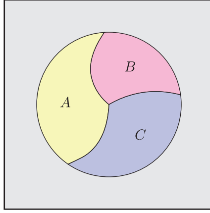
Figure 5.4: Three restricted regions for which \mathcal{Q}_{\text{Kit}} can be calculated. Now there is only one point where the three regions meet. Provided that P remains short ranged in the circular region and the distance from the triple contact point to the boundary of the circle is larger than the correlation length of P , this will calculate a quantised Chern number.
