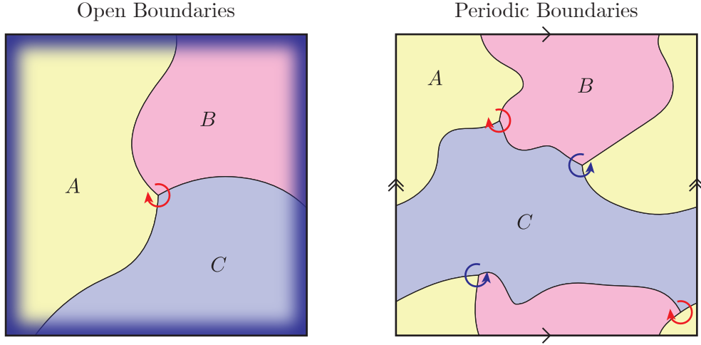
Figure 5.3: Two examples depicting how \mathcal{Q}_{\text{Kit}} vanishes in finite systems. (Left) A topological system in open boundary conditions with necessarily have gapless edge modes present (depicted here with a blue border), which contribute a term to \mathcal{Q}_{\text{Kit}} that exactly cancels out the topological value around the triple contact point. (Right) An example partition of the torus (shown with opposite edges identified) into three regions. In this case, four triple contact points are present. Around each two have the regions arranged clockwise around them and two counter-clockwise, so overall \mathcal{Q}_{\text{Kit}} vanishes.
