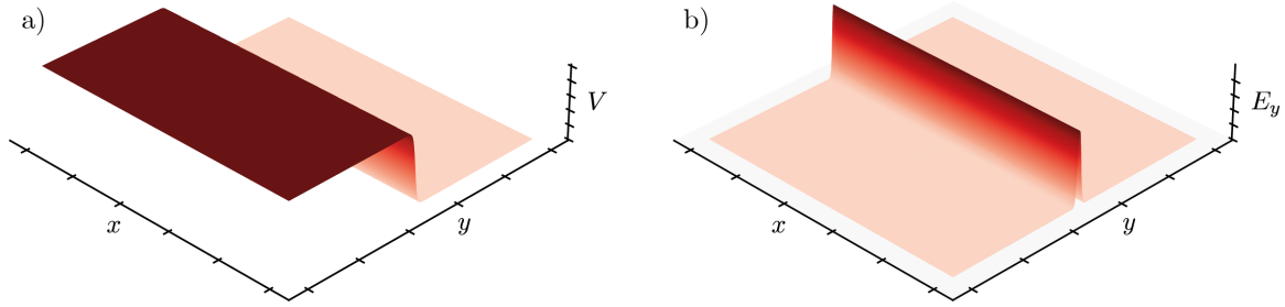
Figure 5.5: a) The electric potential used to generate our electric field. b) The electric field, with only the nonzero y -component is shown.
