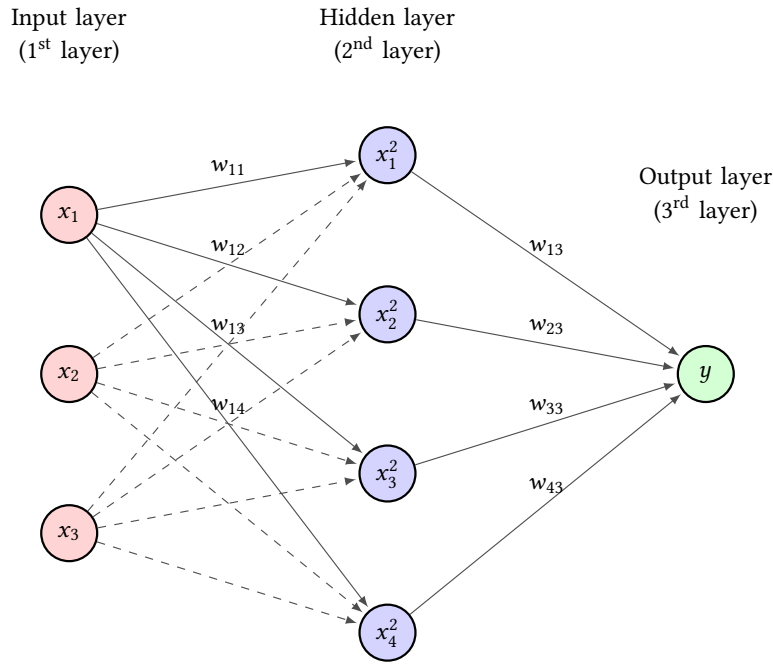
Figure 7.2: Graphical illustration of a single hidden layer ANN, yielding a function from \mathbb{R}^3 to \mathbb{R} . We only made explicit the weights relative to the first variable.
