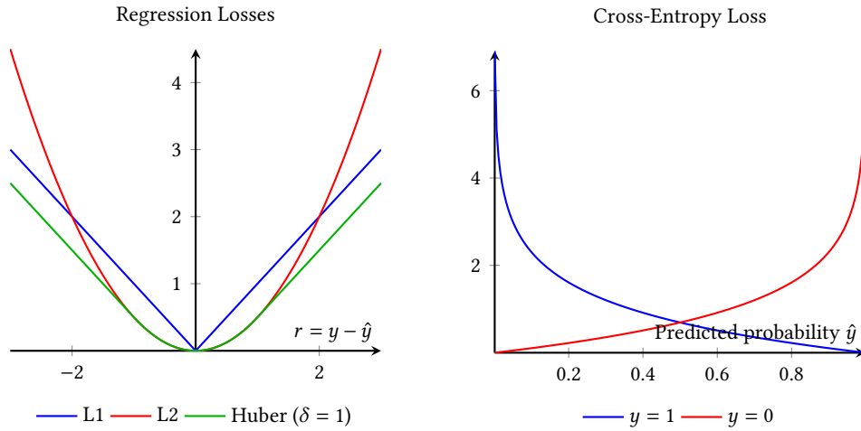
Figure 6.1: Typical loss functions for Y = \mathbb{R} (left) and the cross-entropy loss (right).
