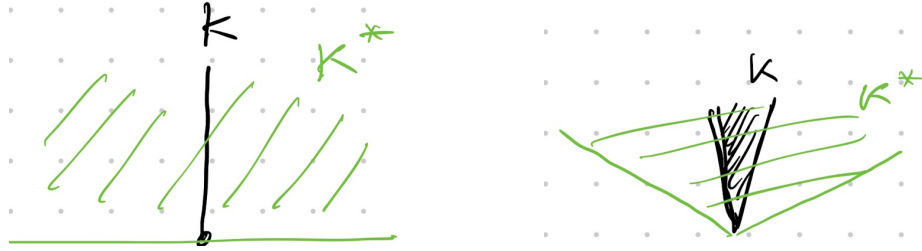
Figure 1.2: Two examples of dual cone.
