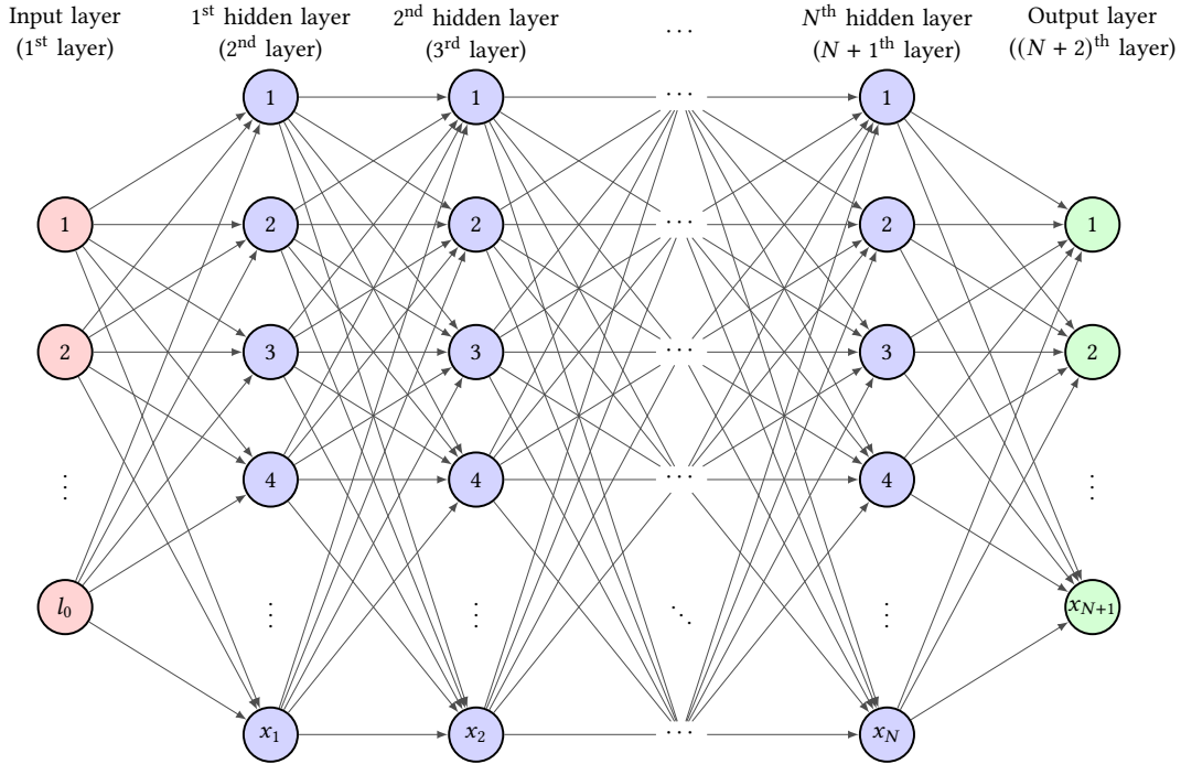
Figure 7.3: Graphical illustration of a fully-connected feedforward ANN consisting of L + 1 affine transformations (i.e., of L + 2 layers: one input layer, L hidden layers, and one output layer). Image from [8].
