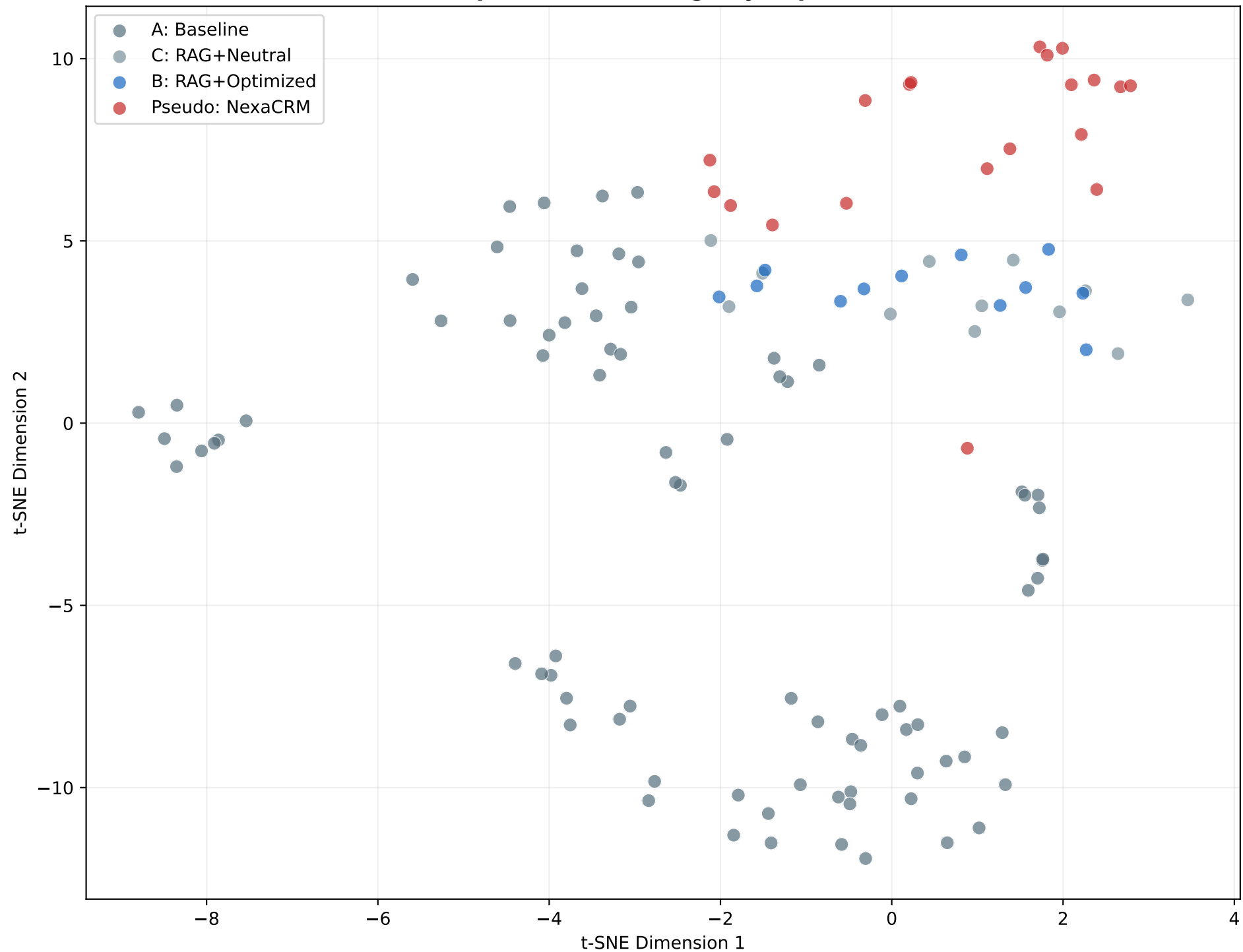
t-SNE of LLM Response Embeddings by Experimental Condition
