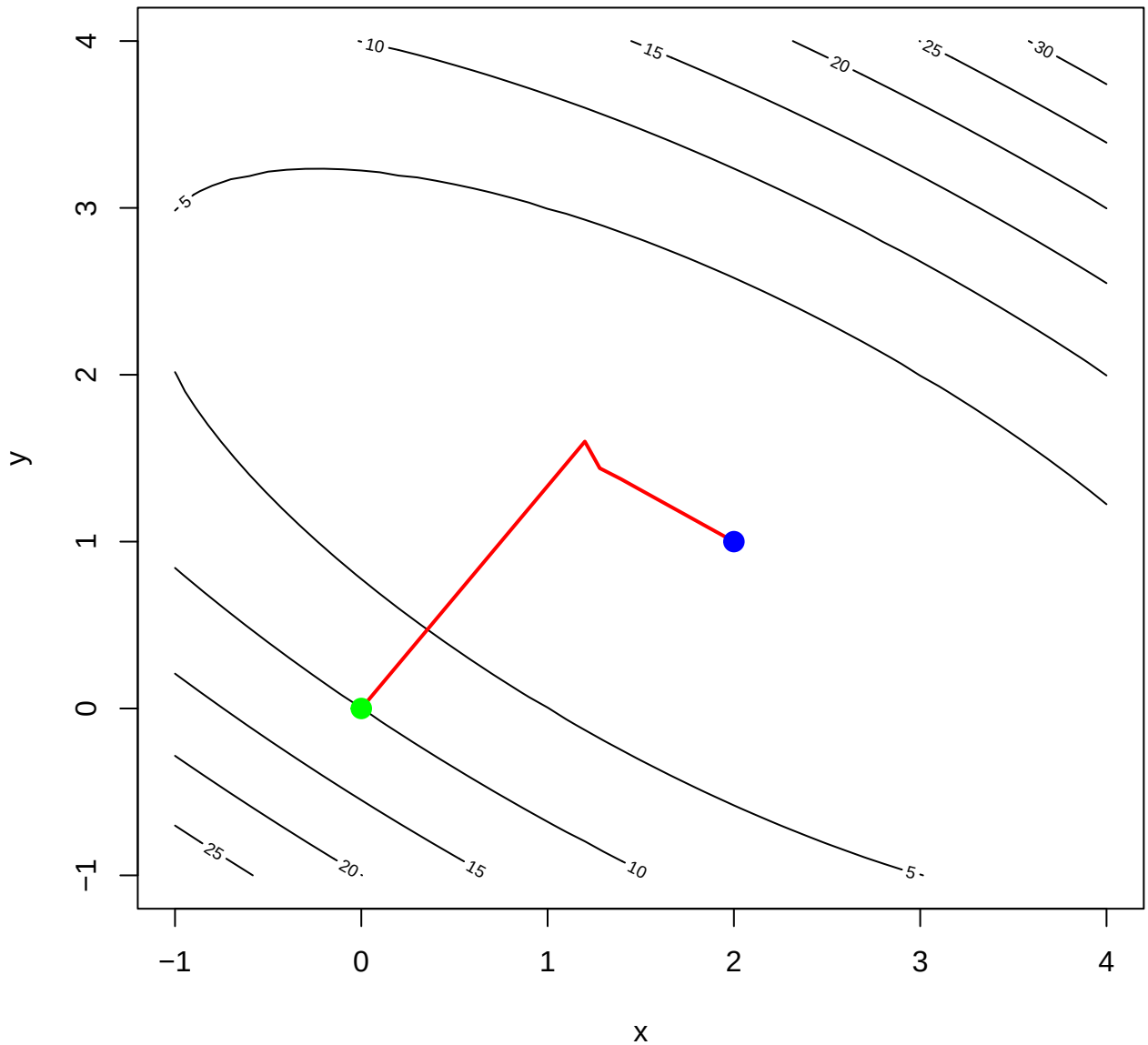
f(x,y) and gradient descent path
