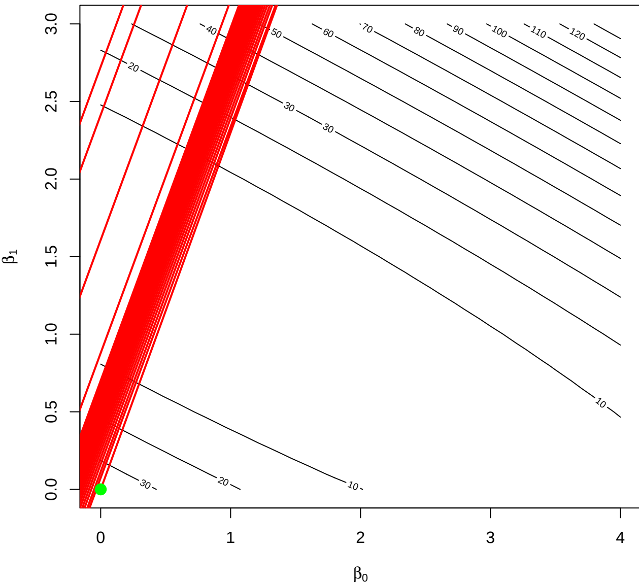
SSE surface and gradient descent path
