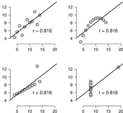
Anscombe's Quartet
