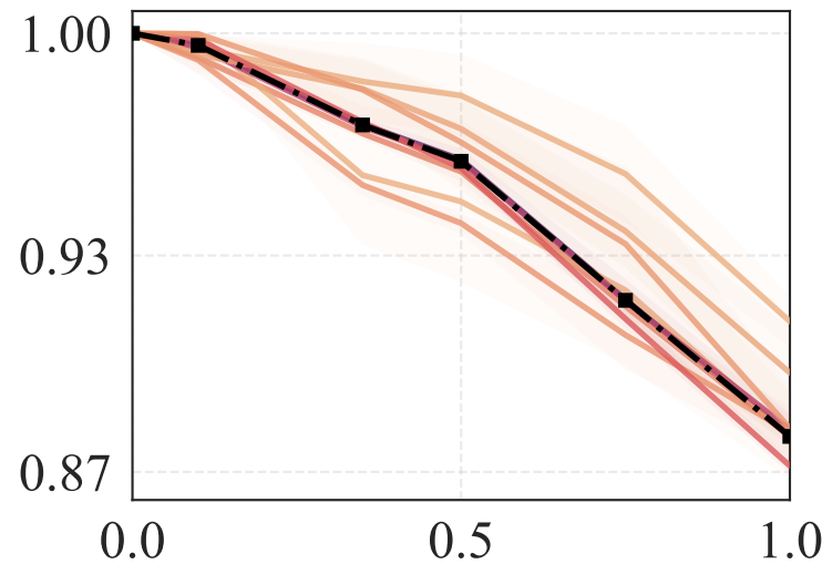
Mean
