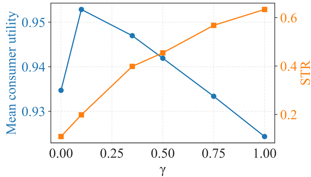
k = 20
