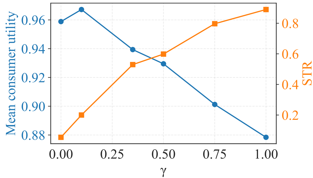
k = 10
