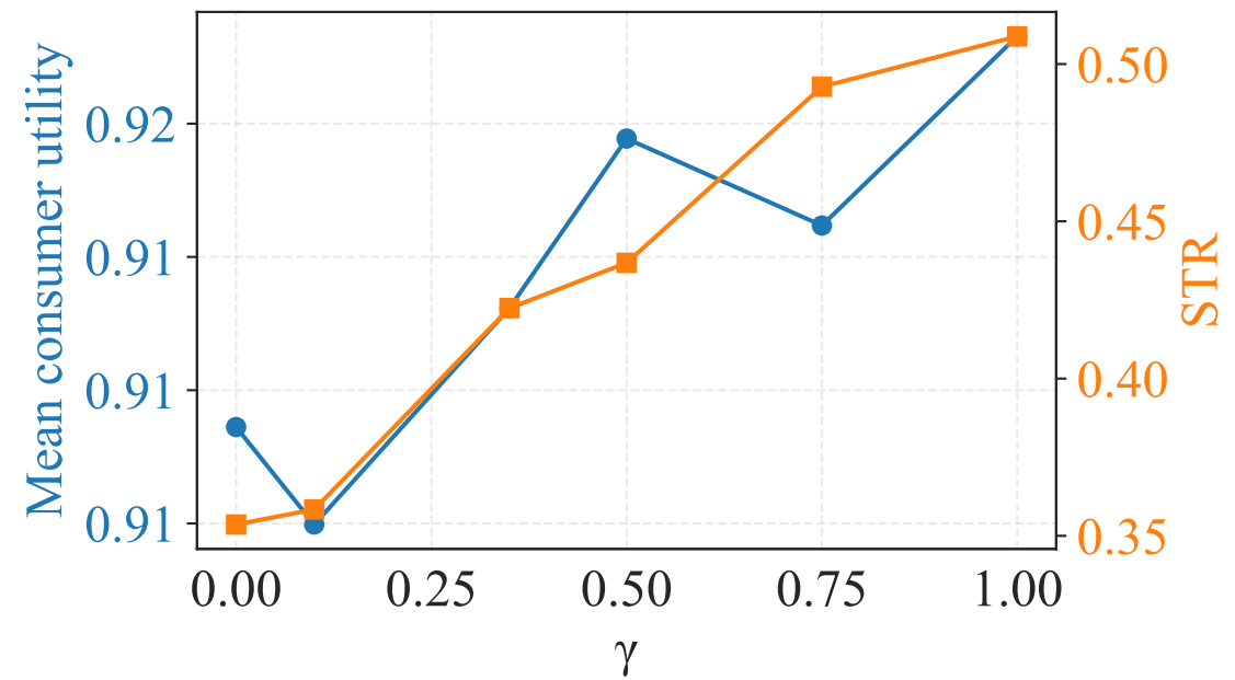
k = 100
