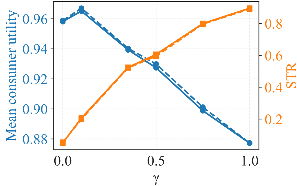
k = 10
