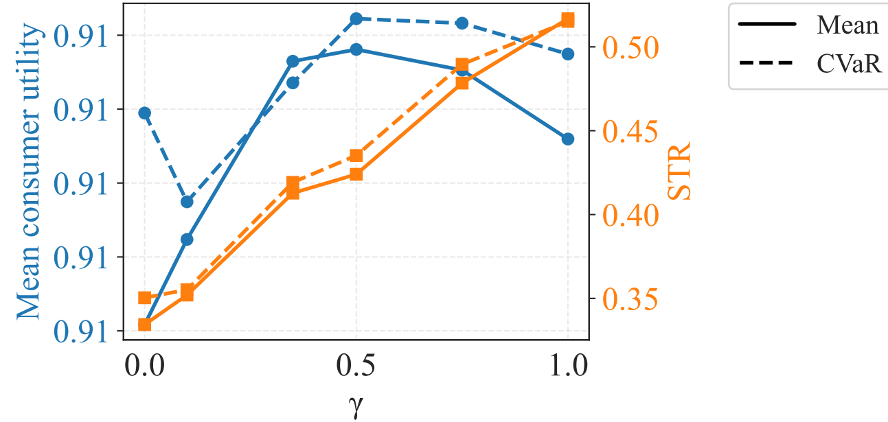
k = 100
