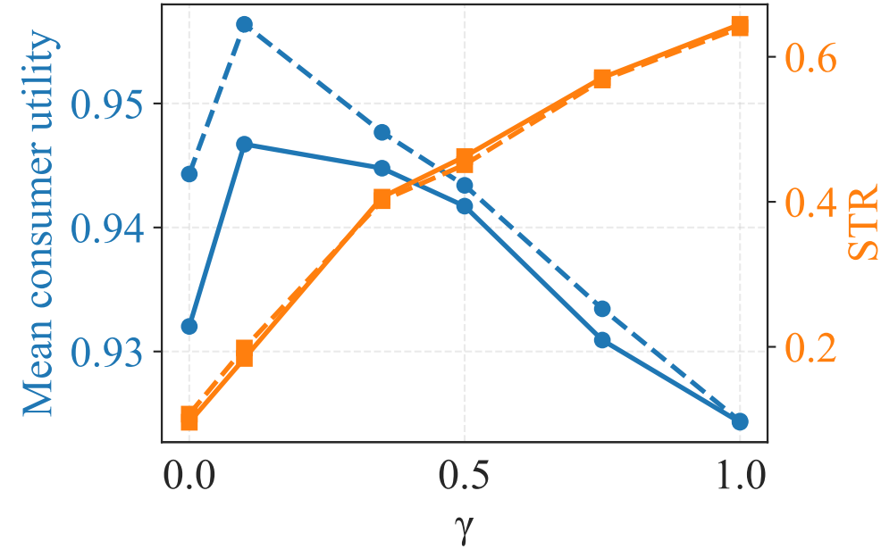
k = 20
