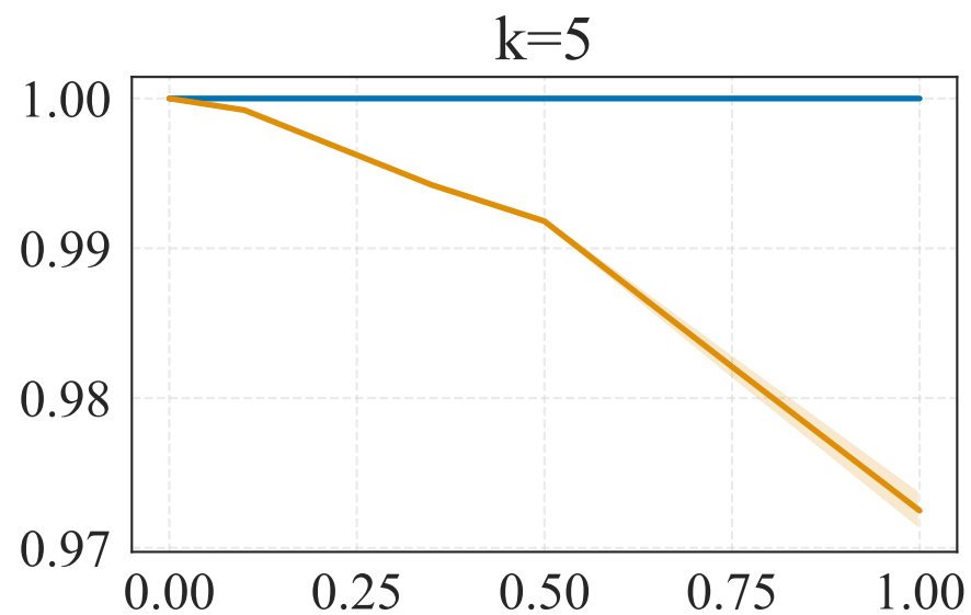
Amazon
