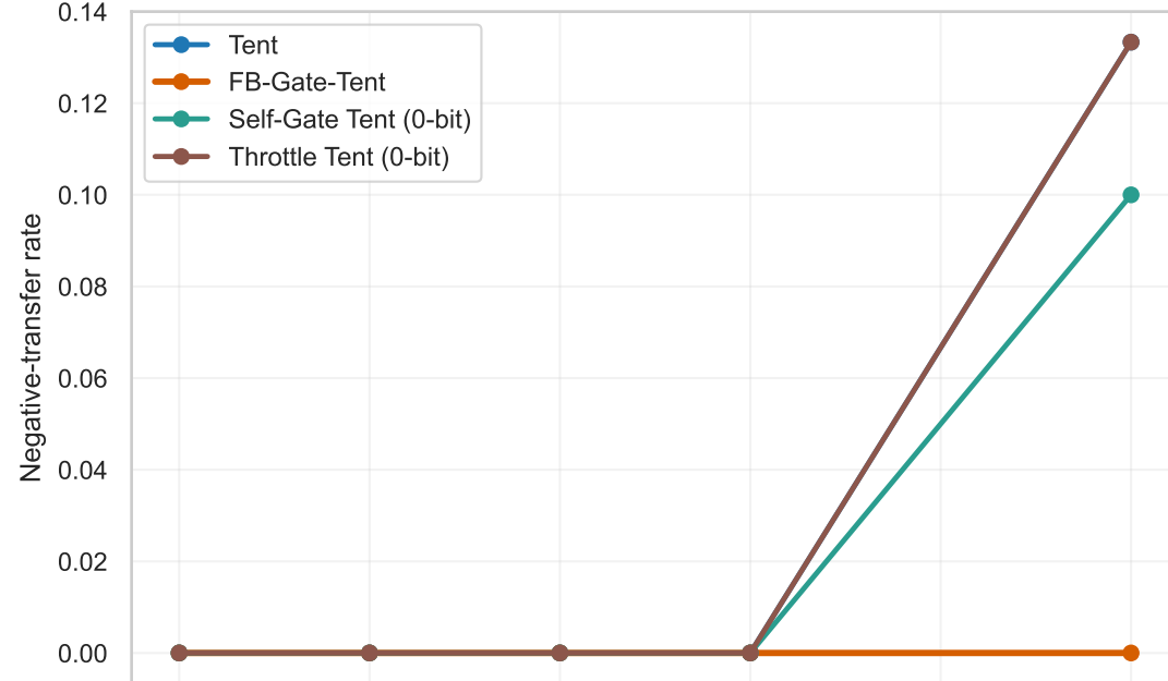
CIFAR-100: negative transfer at q = 0.01
