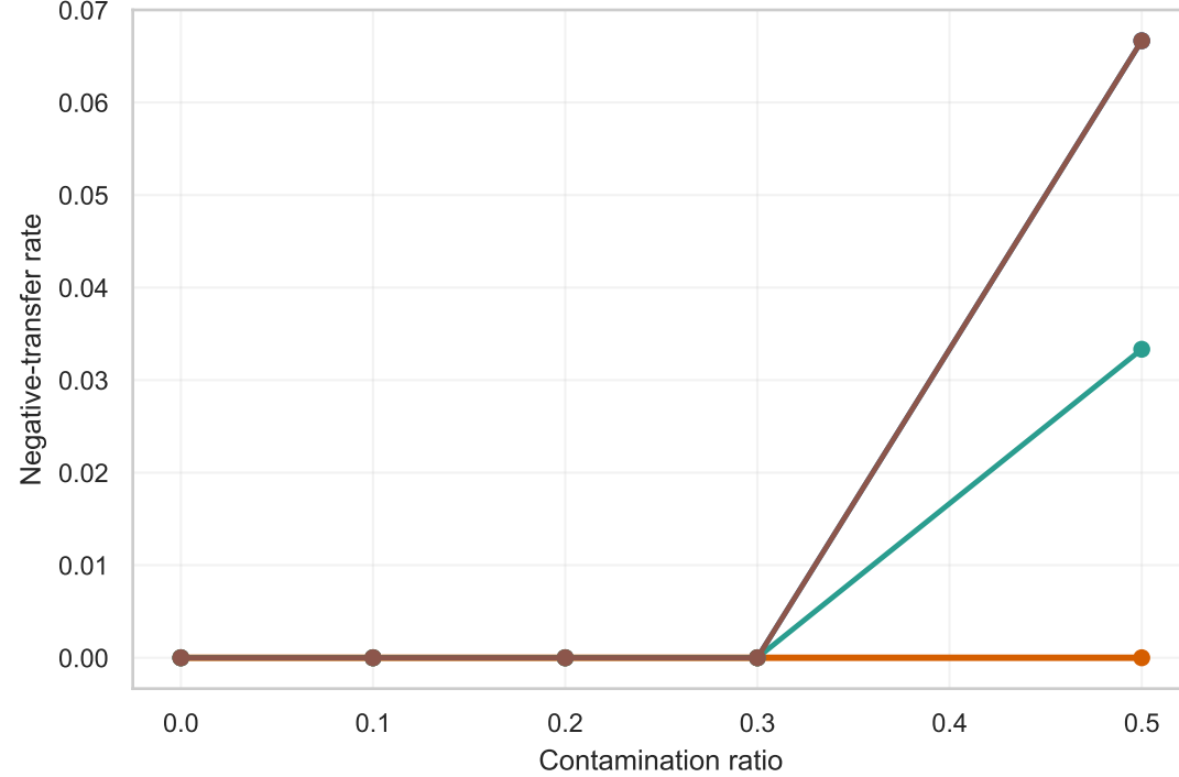
CIFAR-100: negative transfer at q = 0.01
