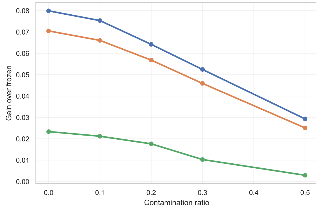
CIFAR-10 delay
