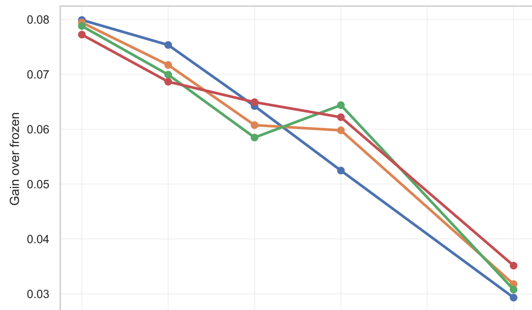
CIFAR-10 delay
