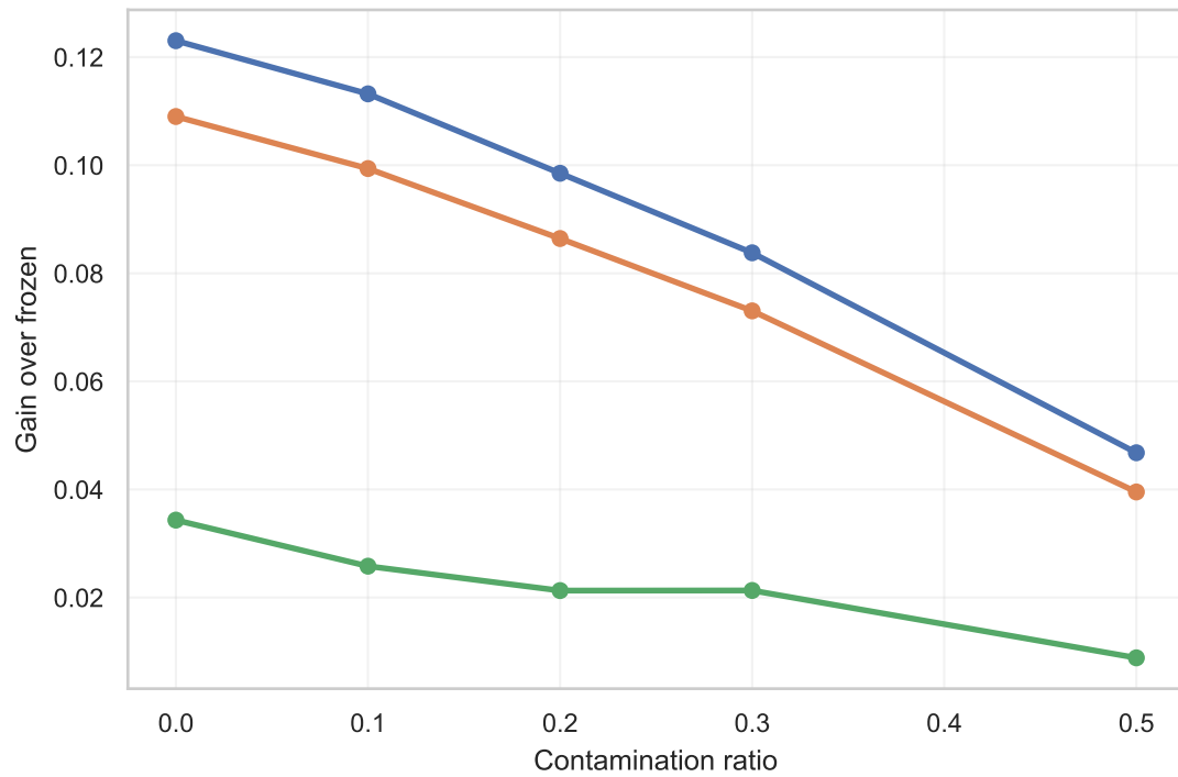
CIFAR-100 delay
