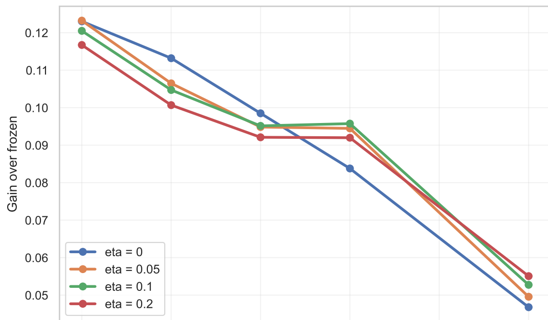
CIFAR-100 delay
