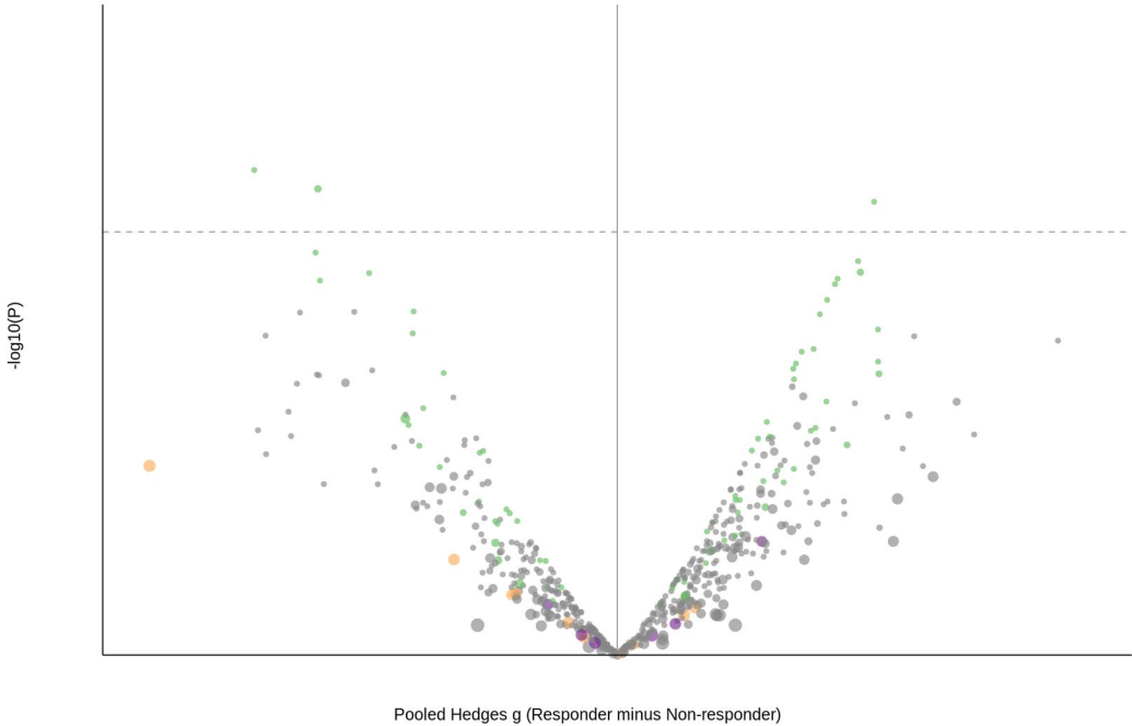
Random-effects meta-analysis of domain-level CLR effects
