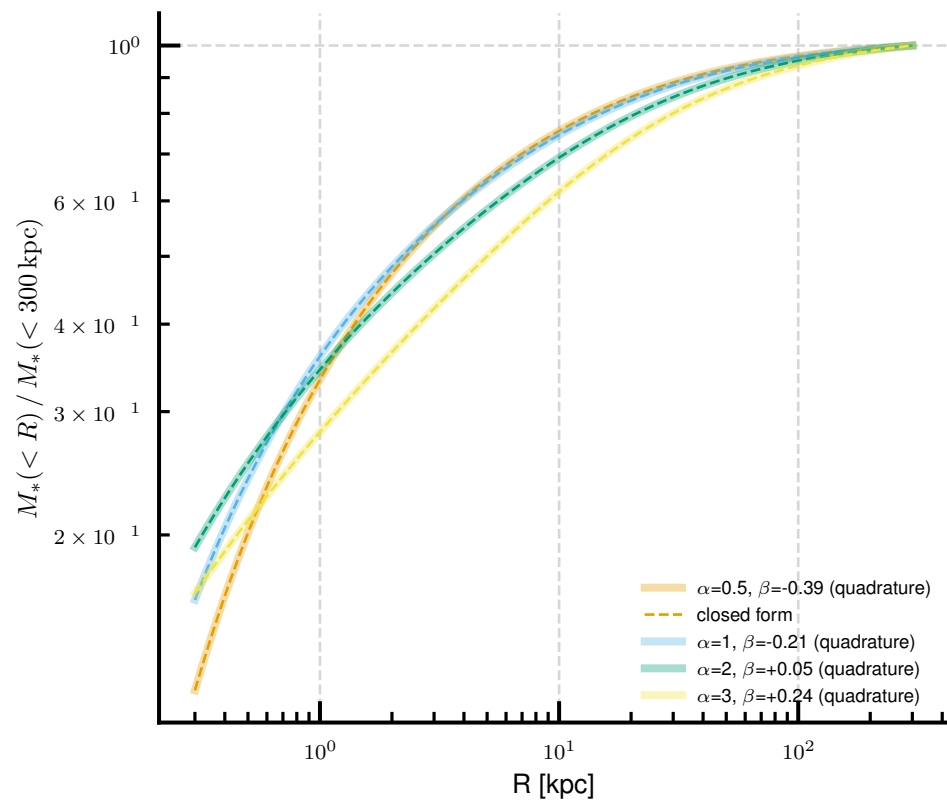
(b) power-law MAH: incomplete-gamma CoG is exact
