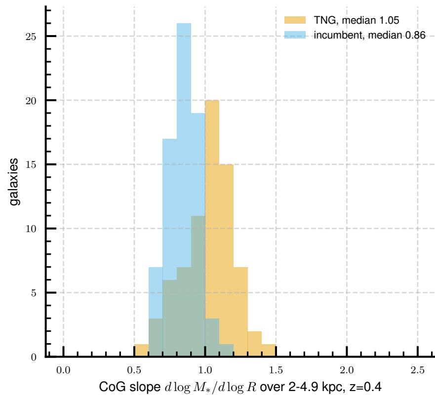
(c) inner slope: the model is shallower and narrower
