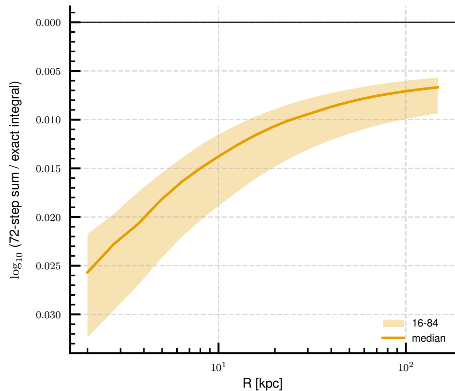
(a) incumbent's discretisation error, z=0.4 (73 galaxies)
