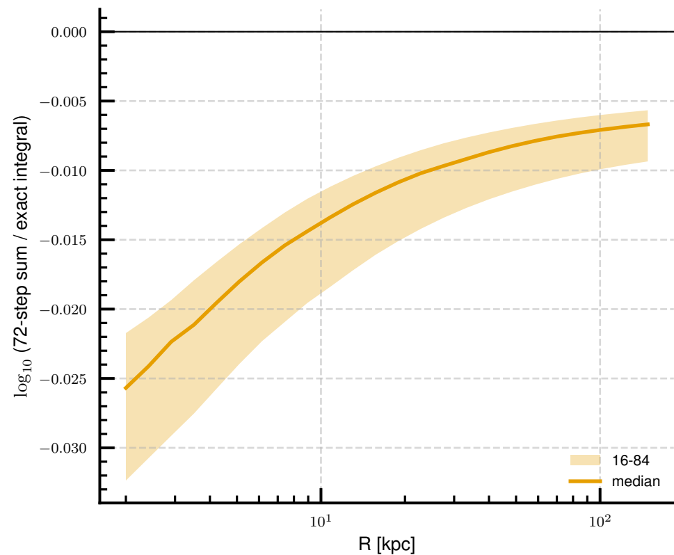
(a) incumbent's discretisation error, z=0.4 (73 galaxies)
