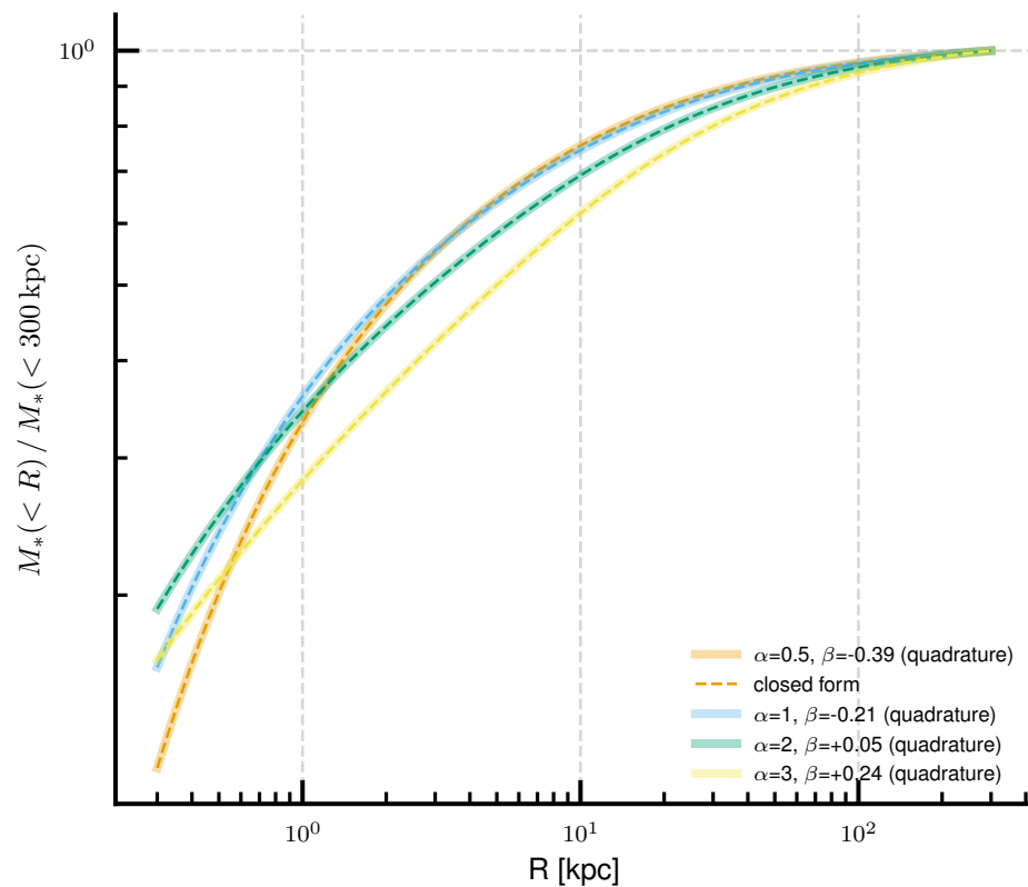
(b) power-law MAH: incomplete-gamma CoG is exact
