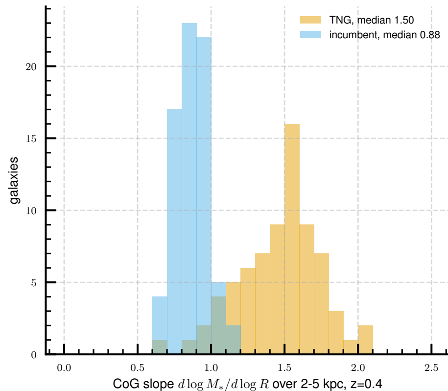
(c) the model's centre rises too slowly
