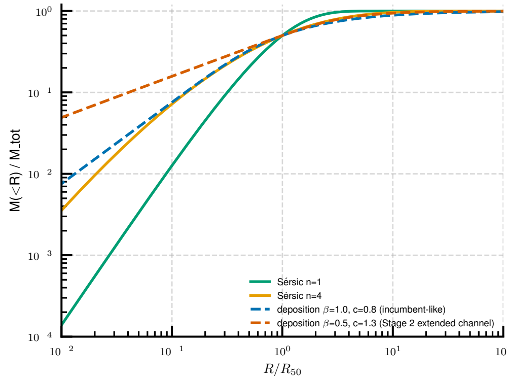
(a) the curves of growth
