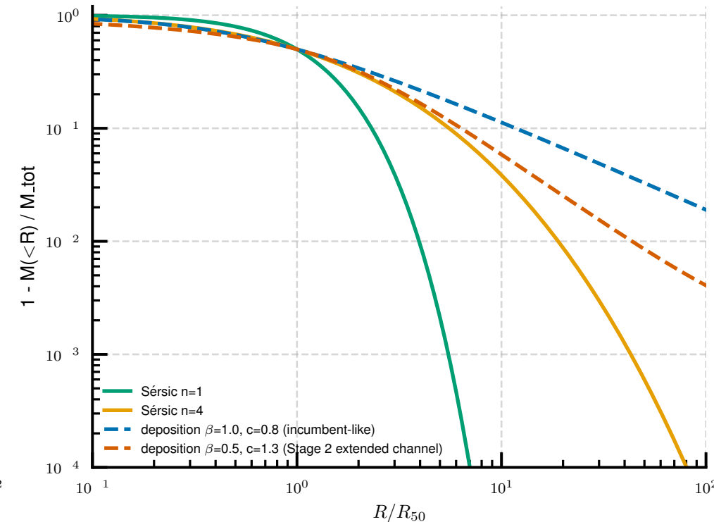
(c) approach to the total: stretched exponential vs power law
