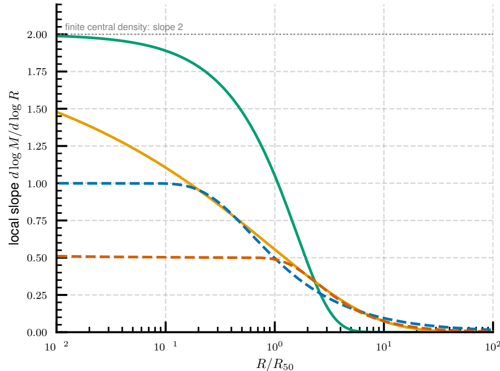
(b) Sérsic starts at 2; deposition starts at \beta
