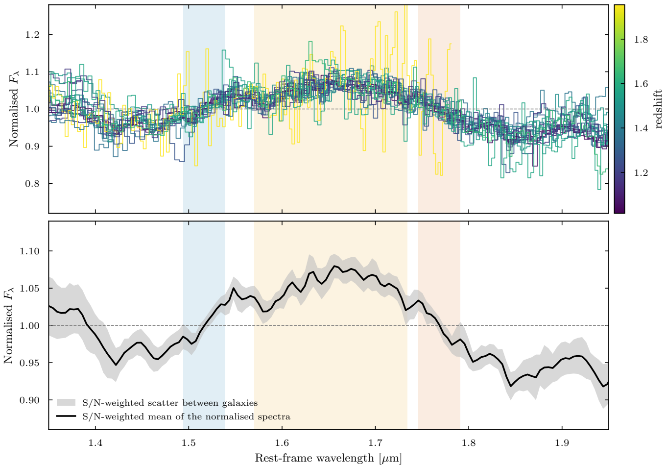
19 JWST PRISM quiescent galaxies (Lu+2026), rest frame
