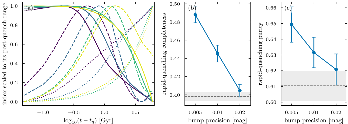
AGB on; (a) tracks at t_q = 3 Gyr, solar metallicity, delayed- \tau rise with \tau = t_q
