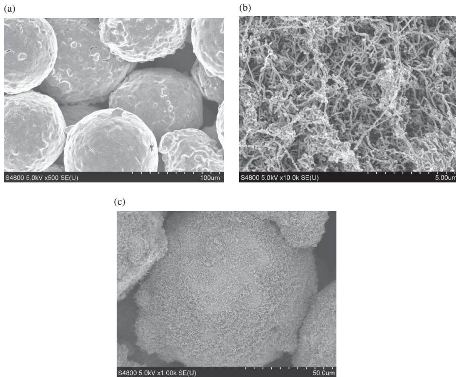
Figure 1 SEM images of boiling surfaces fabricated for this work: (a) porous layer formed of sintered copper spheres, (b) Cu-metallized MWCNT array, and (c) sintered Cu spheres with metallized CNT array grown after sintering.
