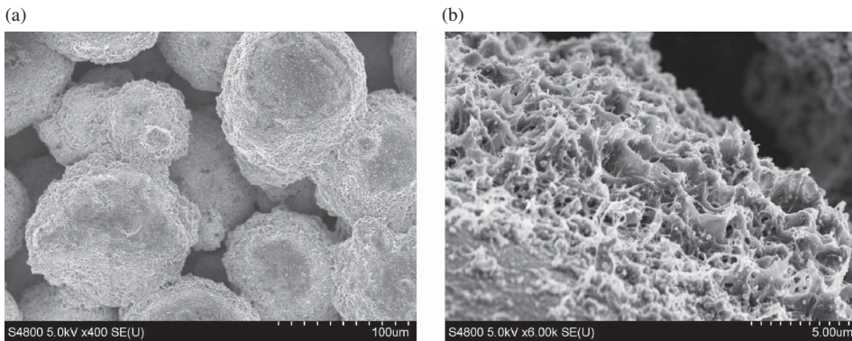
Figure 6 SEM images of the sintered boiling surface after pool boiling tests and desoldering.
