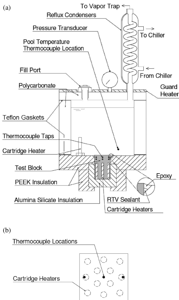
Figure 2 (a) Schematic diagram of the experimental facility with relevant components indicated and (b) top view of the test block (adapted from McHale and Garimella [26]).
