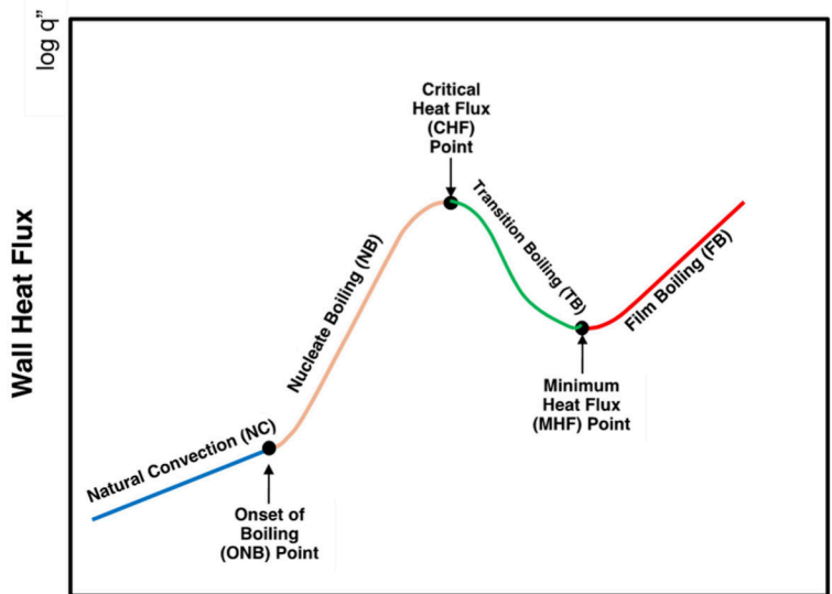
Fig. 1. Boiling curve obtained from (a) heat-flux-controlled experiments and (b) temperature-controlled experiments.
