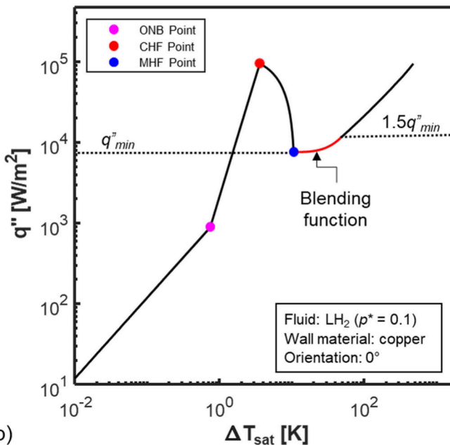
Fig. 2. Complete boiling curve for LH 2 (a) without blending function and (b) with blending function.
