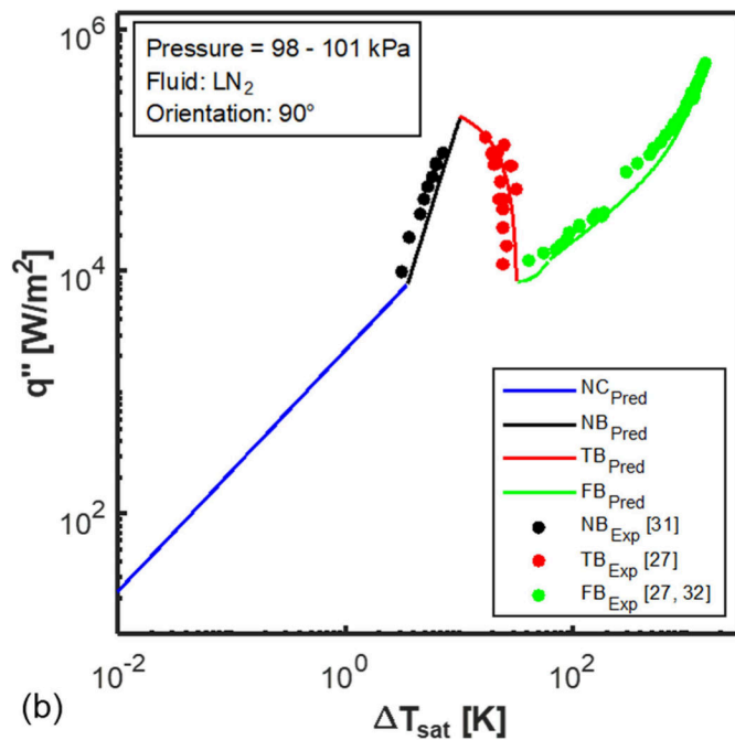
Fig. 6. Validation of new pool boiling curve construction methodology against LN 2 data for (a) horizontal and (b) vertical surface orientations.
