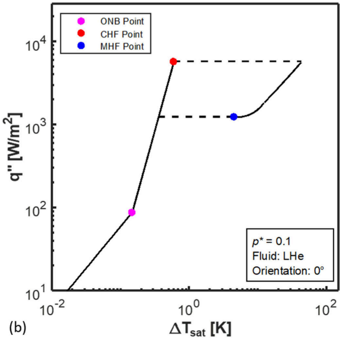
Fig. 7. Comparison of (a) heat-flux-controlled (b) temperature-controlled boiling curve predictions.
