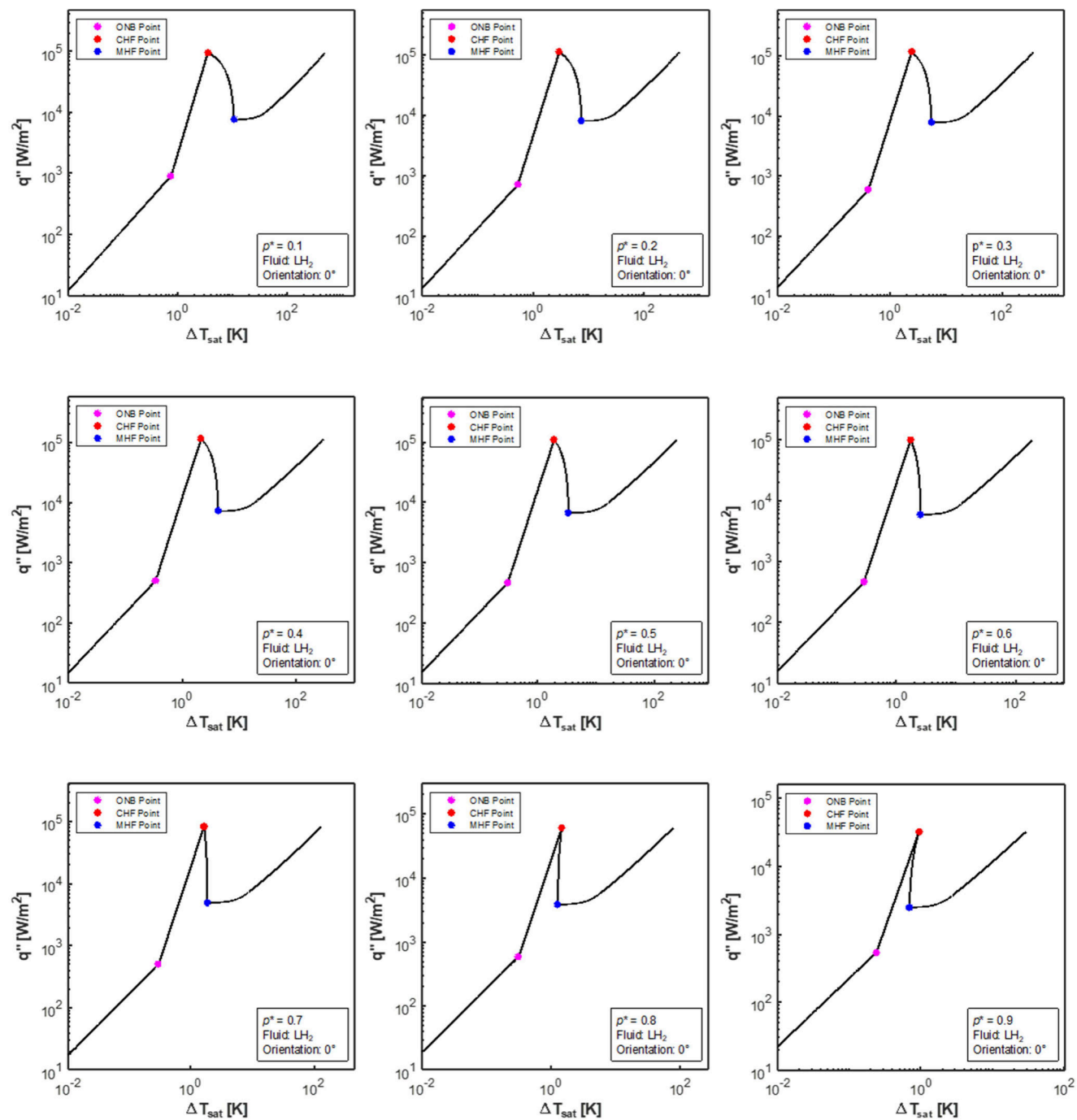
Fig. 8. Predicted continuous boiling curves for \text{LH}_2 for reduced pressures from p^* = 0.1 to 0.9.
