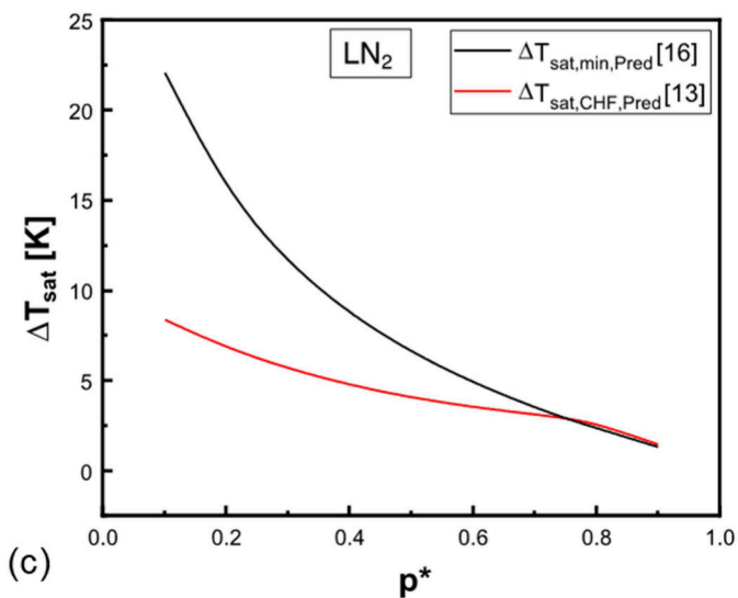
Fig. 9. CHF and MHF superheat predictions versus reduced pressure for (a) LHe (along with experimental data), (b) LH 2 , and (c) LN 2 .
