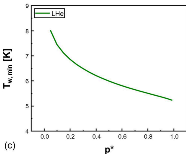
Fig. 10. Variation of minimum wall temperature with reduced pressure according to the baseline correlation [15] for (a) \text{LN}_2 , (b) \text{LH}_2 , and (c) \text{LHe} .
