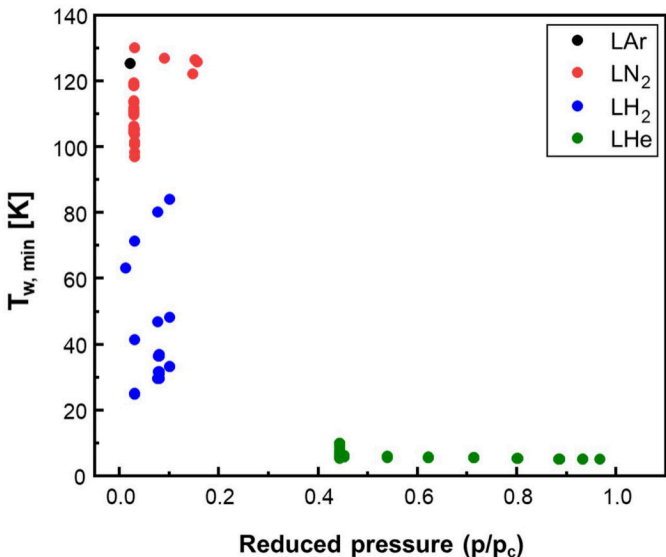
Fig. 11. Variation of minimum wall temperature with reduced pressure for different cryogenes. (Data taken from Ahmad et al. [15] consolidated T_{\min} database).
