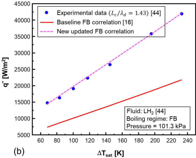
Fig. 15. (a) LN 2 FB data from [43] for different heated surface sizes, (b) FB predictions based on baseline and newly updated correlations compared to LH 2 data from [44].
