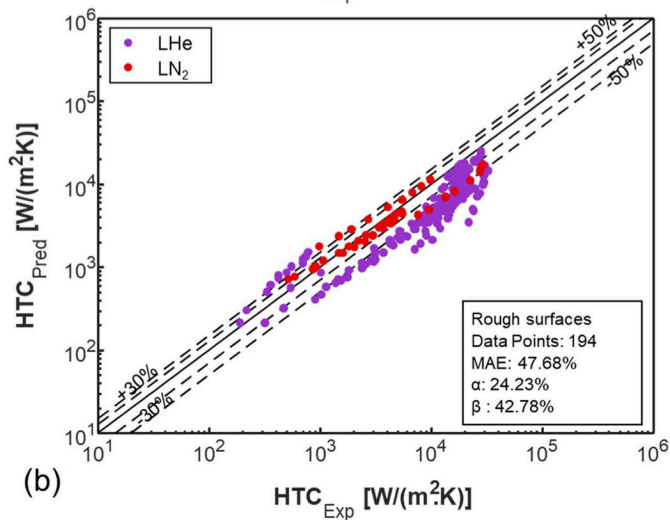
Fig. 3. Predictions of the baseline NB HTC correlation [11] against data for (a) smooth surfaces and (b) rough surfaces. (Data taken from Ahmad et al. [11] NB consolidated database).
