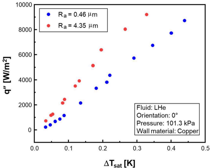
Fig. 4. NB heat flux versus wall superheat for LHe for rough surfaces with different R_a values. (Data taken from [27]).
