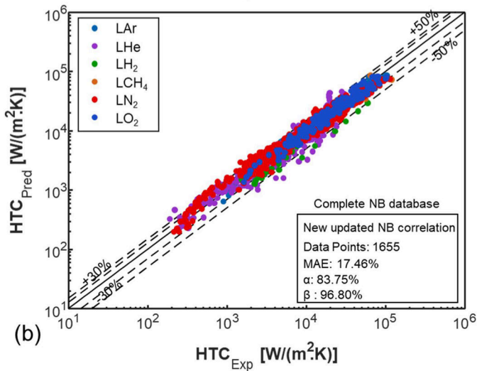
Fig. 7. Predictions of (a) baseline NB HTC and (b) updated NB HTC for complete cryogenic database. (Data taken from Ahmad et al. [11] NB consolidated database).
