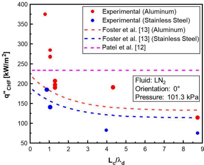
Fig. 9. Variation of CHF for LN 2 with heater characteristic length normalized by Taylor's most dangerous wavelength compared to predictions of correlations by Patel et al. [12] and Foster et al. [13]. (Data taken from the consolidated CHF database of Patel et al. [12] and Foster et al. [13]).
