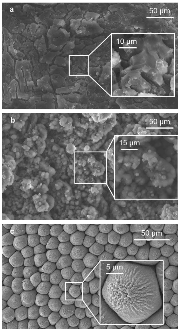
Figure 1. Scanning electron microscope images of the aluminum textured surfaces fabricated in this study.
