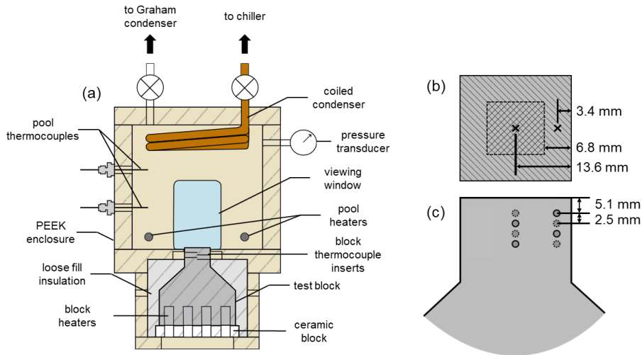
Figure 2. Schematic illustration of (a) the pool boiling test facility and (b)-(c) test block. (b) top-down view
