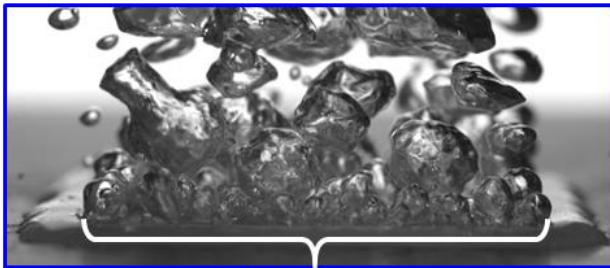
dense nucleate boiling across surface
