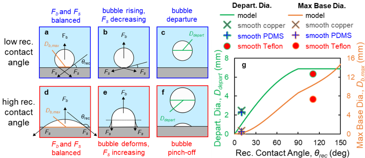
Figure 6. Illustration of approximate bubble growth progressions and results of bubble growth model.
