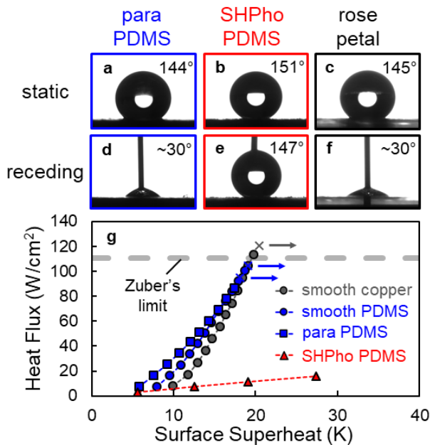
Figure 7. Wettability characterization and boiling results for textured PDMS-coated surfaces. Static 5 \mu\text{L}
