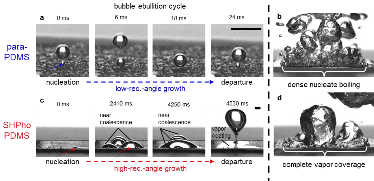
Figure 8. Comparison of the bubble ebullition cycle and boiling behavior of the textured PDMS-coated
