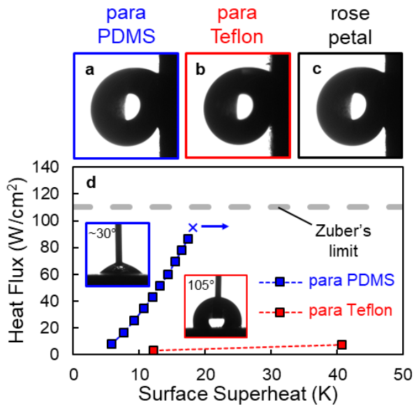
Figure 9. Wetting behavior and boiling results for parahydrophobic PDMS-coated (para PDMS) and
