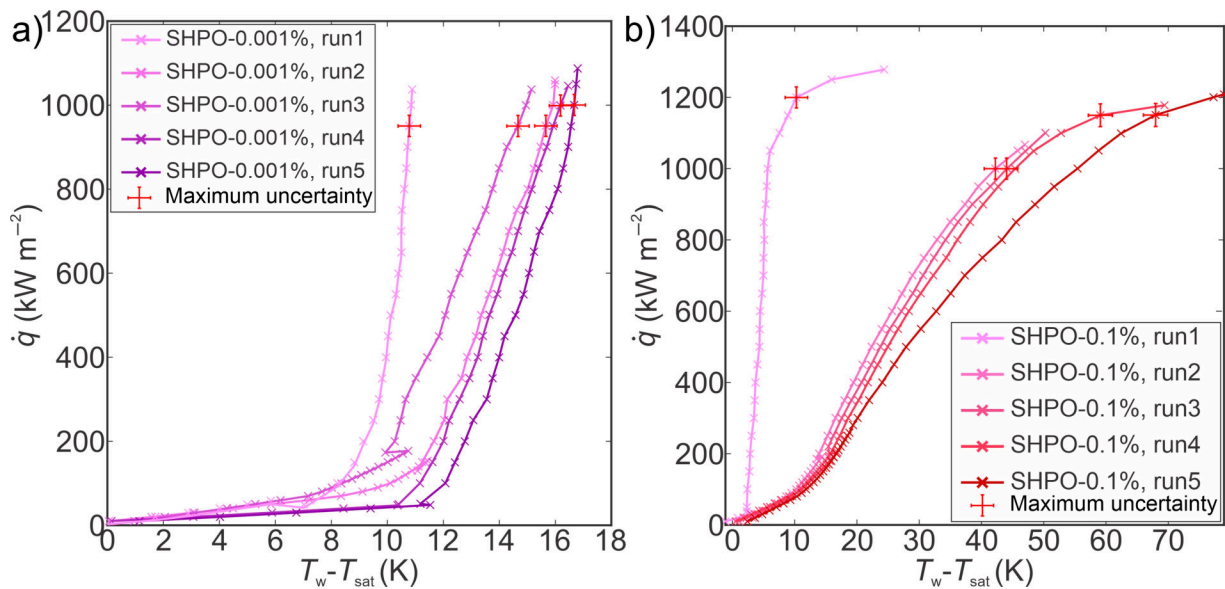
Figure 10. Boiling curves of TiO 2 -water nanofluid on a superhydrophobic laser-textured surface at (a) 0.001 wt.% and (b) 0.1 wt.% concentrations of TiO 2 nanoparticles.
