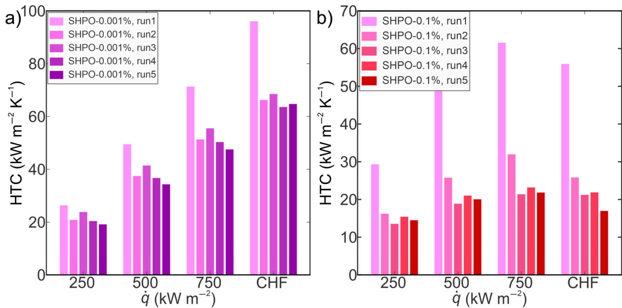
Figure 11. Heat transfer coefficients of \text{TiO}_2 -water nanofluid on a superhydrophobic laser-textured surface at (a) 0.001 wt.% and (b) 0.1 wt.% concentrations of \text{TiO}_2 nanoparticles.
