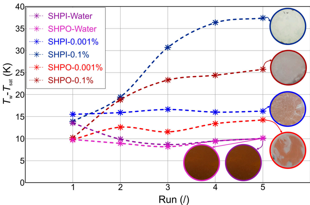
Figure 13. Nanoparticle deposition-induced changes, characterized by mean pool boiling curve wall temperature in the heat flux range of 50–900 kW m -2 and corresponding sample surface images. Plots of samples boiled in clean water are included to serve as a reference and point out that boiling performance also changes in clean water, where no deposition was observed.
