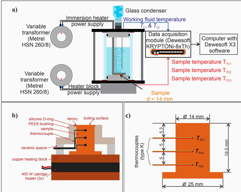
Figure 2. (a) Experimental setup; (b) cross section of the sample and the heating assembly; and (c) dimensions of the sample, including the position of thermocouples.
