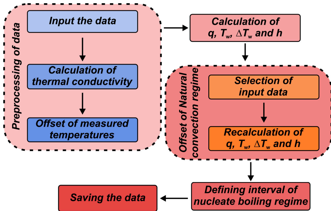
Figure 3. Flowchart of processing the data obtained during pool measurements.
