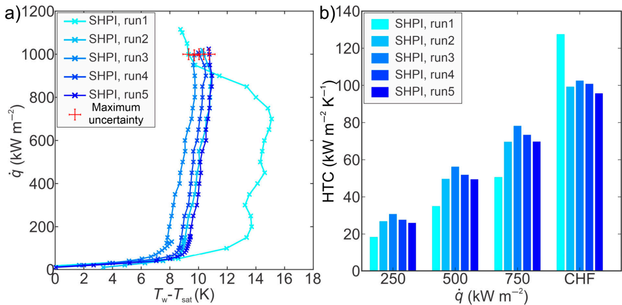
Figure 5. (a) Boiling curves and (b) heat transfer coefficients on the superhydrophilic laser-textured surface.
