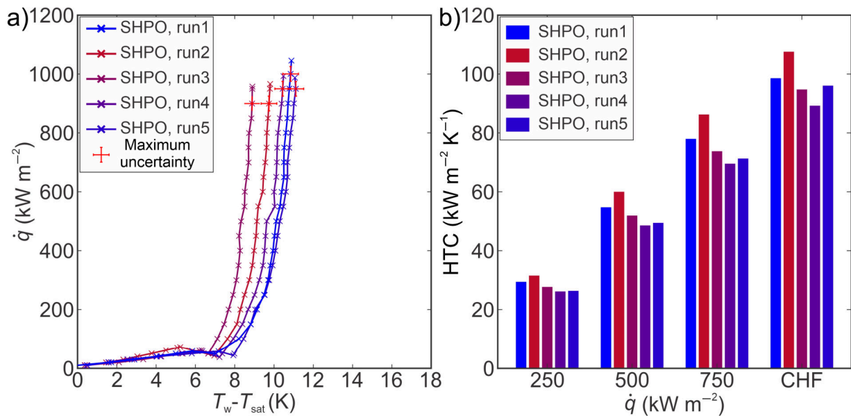
Figure 6. (a) Boiling curves and (b) heat transfer coefficients on the superhydrophobic laser-textured surface.
