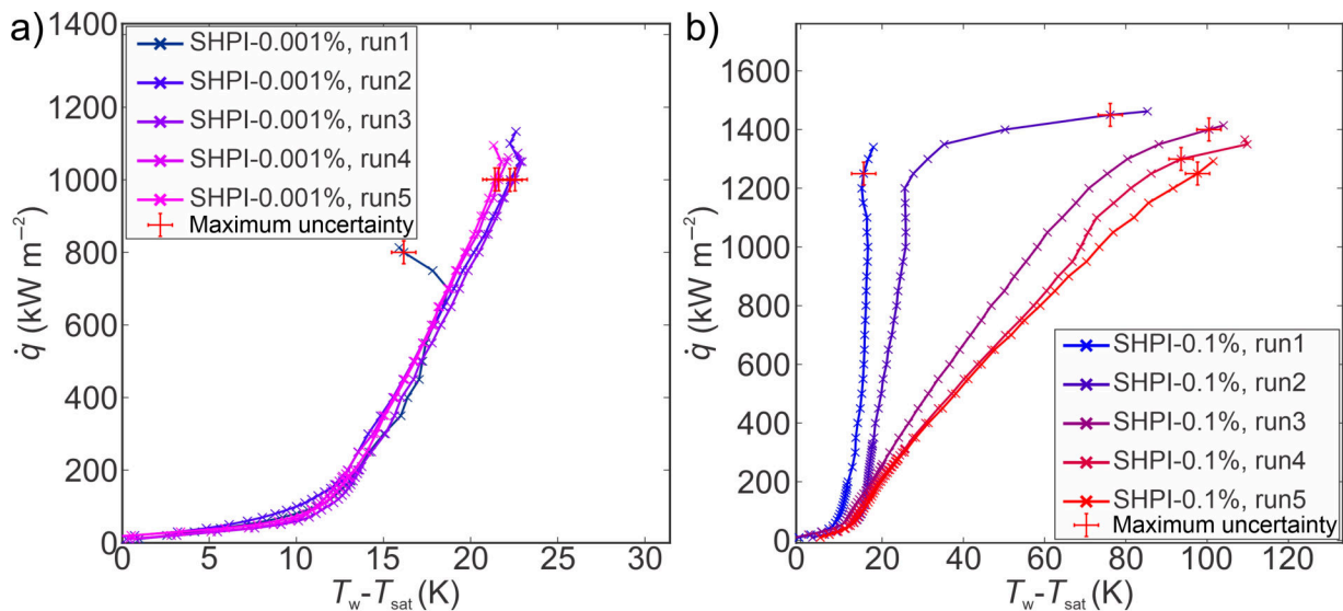
Figure 7. Boiling curves of TiO 2 -water nanofluid on a superhydrophilic laser-textured surface at (a) 0.001 wt.% and (b) 0.1 wt.% concentrations of TiO 2 nanoparticles.
