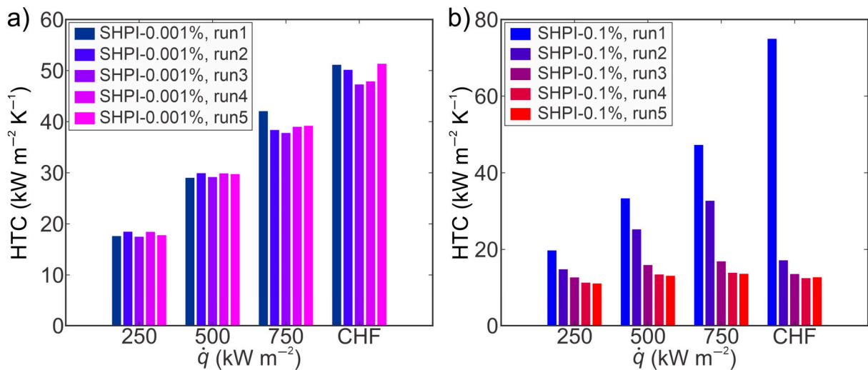
Figure 8. Heat transfer coefficients of \text{TiO}_2 -water nanofluid on a superhydrophilic laser-textured surface at (a) 0.001 wt.% and (b) 0.1 wt.% concentrations of \text{TiO}_2 nanoparticles.
